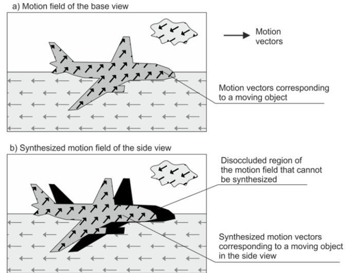
Fig. 9. Independent derivation of motion information for each point of encoded CU from a corresponding point in the reference view.
