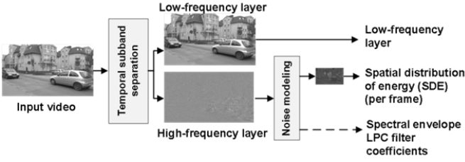
Fig. 7. High-Frequency Layer Representation in an encoder.
