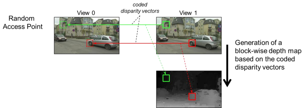
Figure 8: Generation of an initial depth map estimate after coding the first dependent view of a random access unit.
