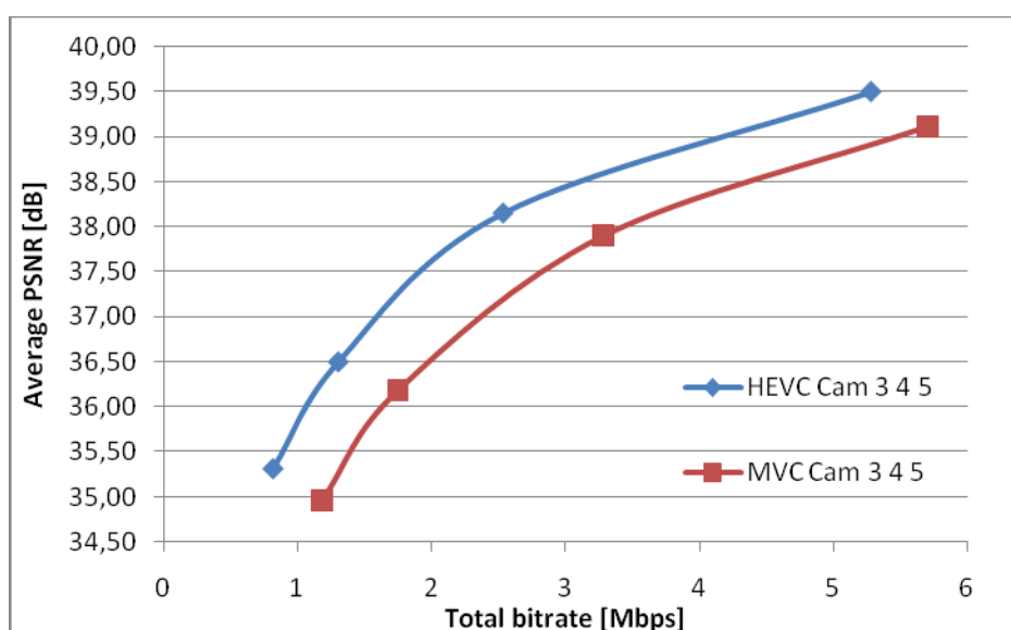
Fig 8. Results of coding three view case for texture video only.
