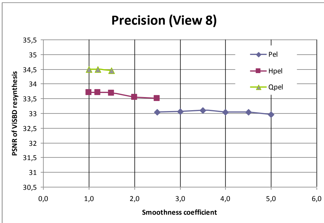
Figure 11. Comparison of matching precision in depth estimation software: full-pixel (Pel), half-pixel (Hpel) and quarter-pixel (Qpel) with respect to resynthesis (ViSBD, splatting “off”) of View 8.
